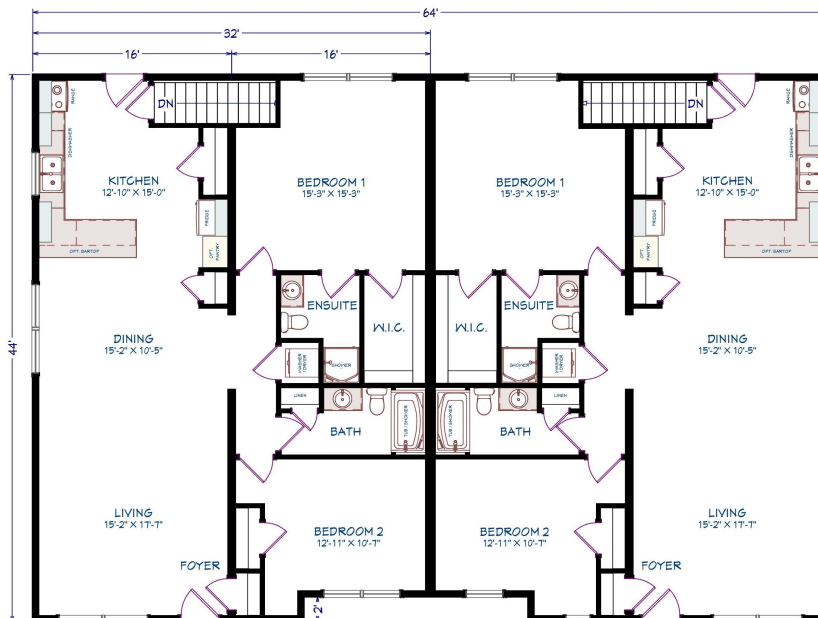
MAIN FLOOR 1 LEVEL DUPLEX, 2 BEDROOM UNITS 1387 SQ FT
