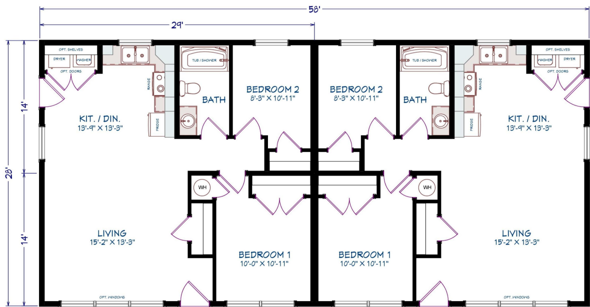
MAIN FLOOR 1 LEVEL DUPLEX, 2 BEDROOM UNITS 812 SQ FT
